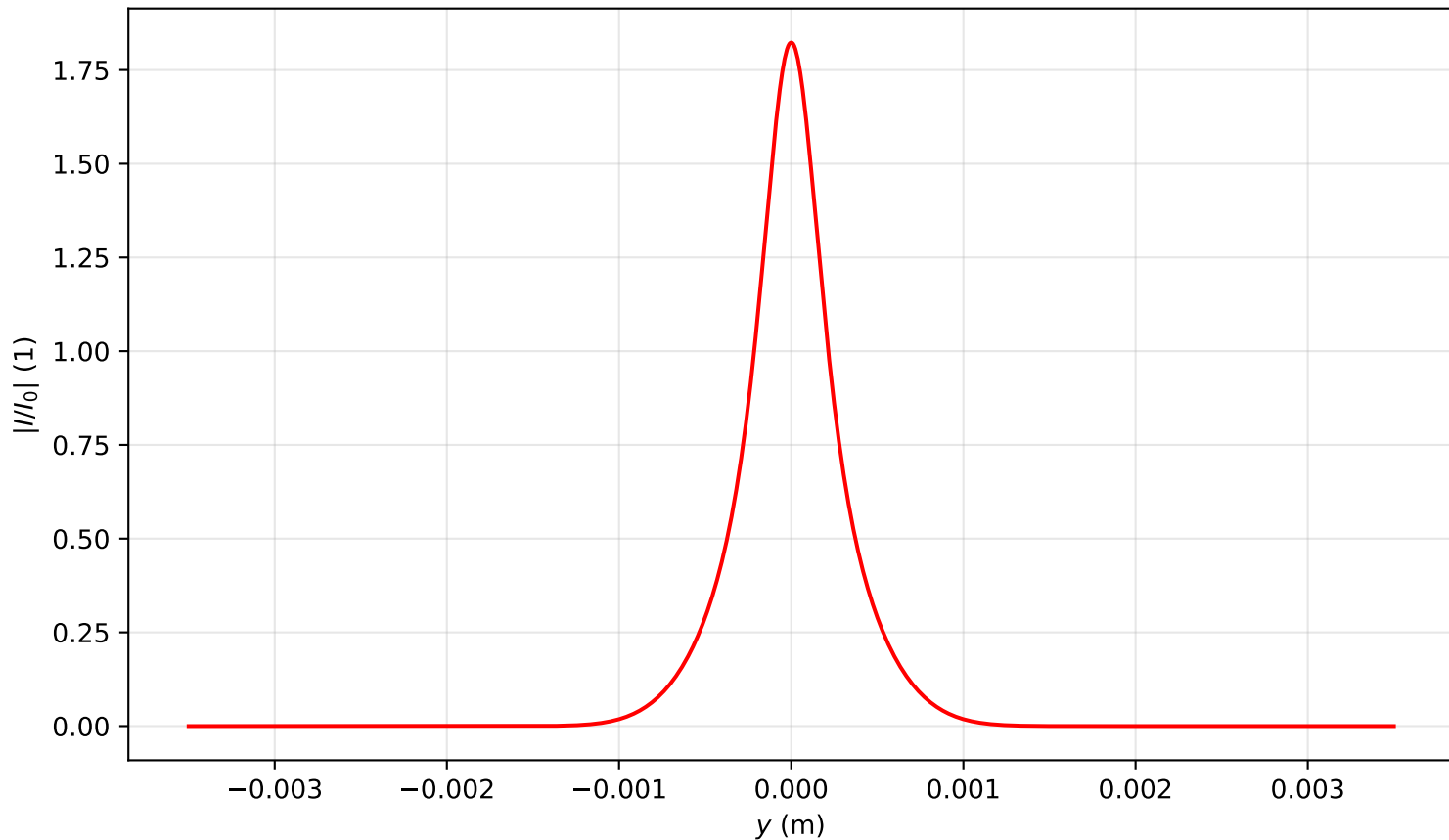
Intensity profile I(x=0, y, z=0.478)/I_0 , P_{in}=2.5P_{cr} , artificial time
